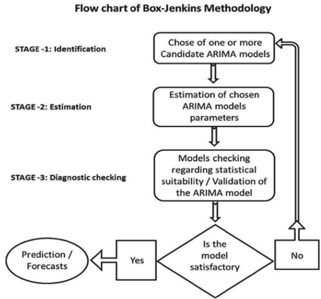
Fig. 1: Flow chart of Box-Jenkins methodology for time series ARIMA model
