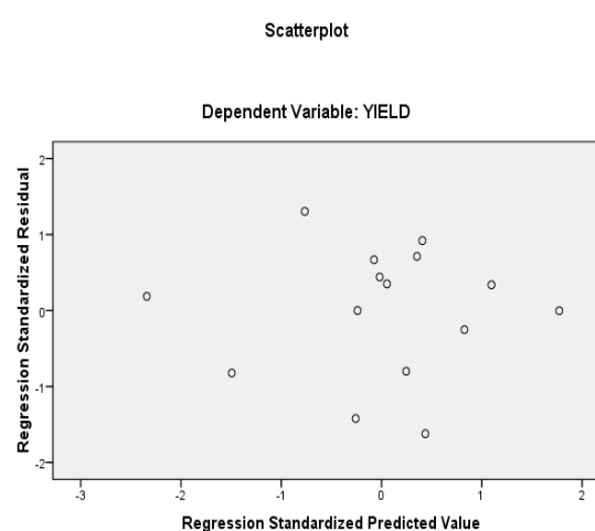
Fig. 4: Residuals scatterplot testing homoscedasticity (Nainital)
