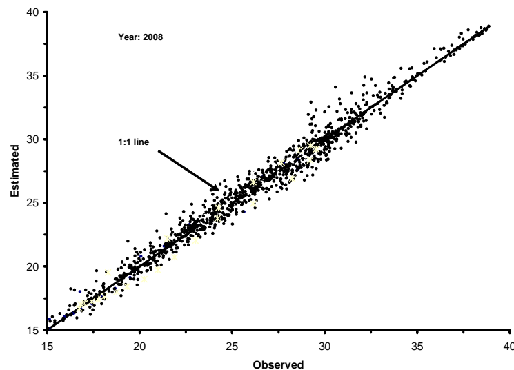
Fig. 2: Observed vs model (sinusoidal/exponential) diurnal temperature ( ^{\circ}\text{C} ) on weekly basis at, Hyderabad
